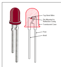
Figure 28 - led's
