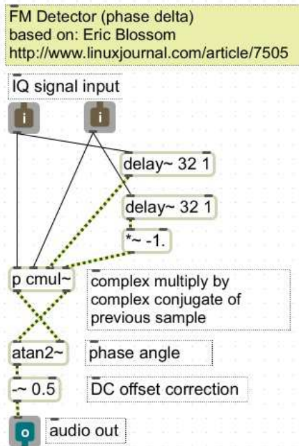
Figure 15 - FM detector
